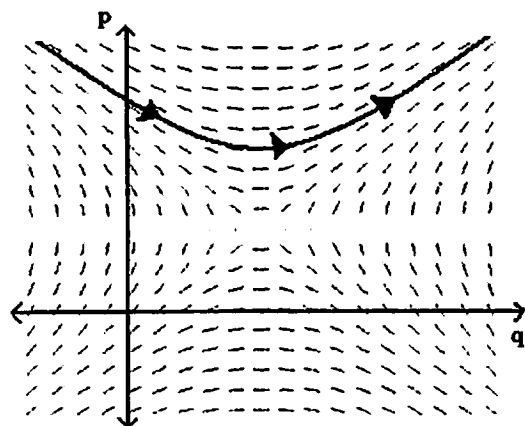
FIG. 2. A Hamiltonian vector field.
