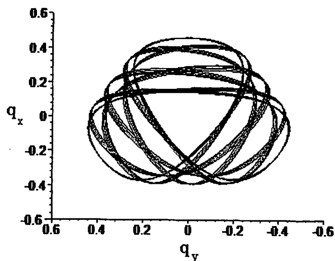
FIG. 3. A solution to the Hénon-Heiles system in the q_y - q_x plane.
