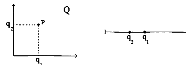
FIG. 1. The configuration space (left) for a two-particle system (right).
