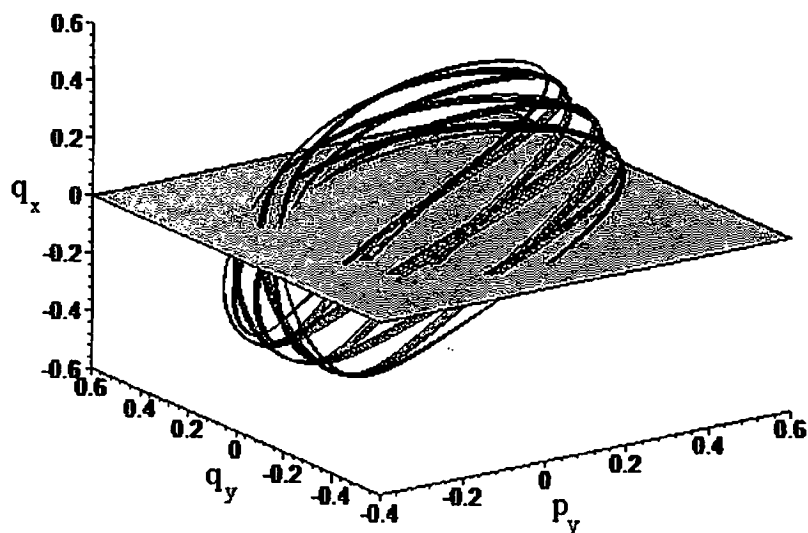
FIG. 4. A solution to the Hénon-Heiles system in the q_y - p_y - q_x volume.
