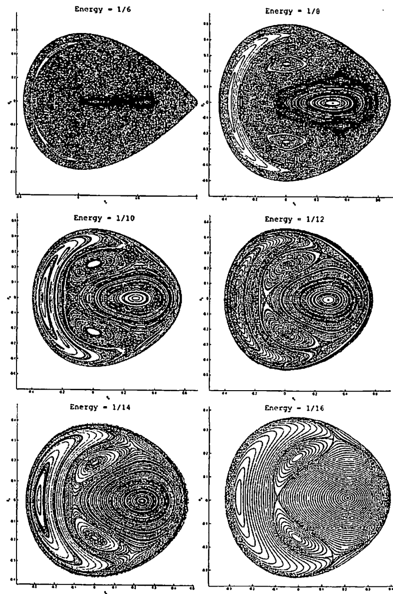
FIG. 6. For high energy ( E = 1/6 ), nearly all of the dynamic states are chaotic. As the energy decreases ( E = 1/8 \rightarrow E = 1/14 ) the regions of chaotic dynamic states shrink, until nearly all dynamic states are regular and predictable ( E = 1/16 ).
