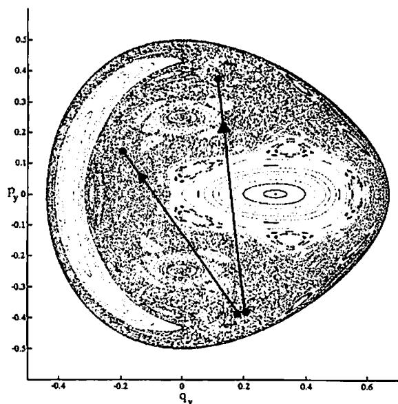
FIG. 5. Two nearby chaotic dynamic states are mapped away from each other.
